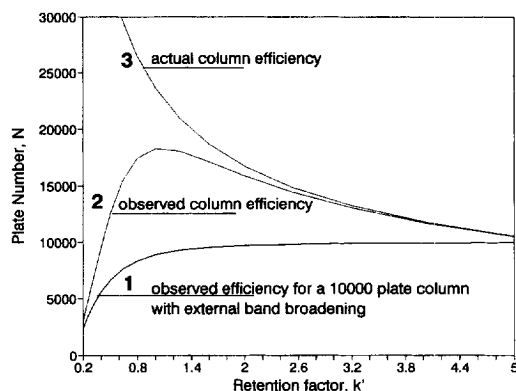
Fig. 1. Efficiency experimental measurement. (1) Observed efficiency for a 10 000 plate column, the extra-column band broadening is heavy in decreasing the column efficiency for low k' solutes, (2) observed efficiency with extracolumn band broadening and efficiency enhancement combined with k' reduction, a maximum N value seems to exist, (3) true column efficiency when enhancements are used in MLC.
