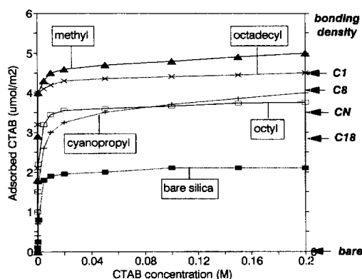
Fig. 4. Amount of adsorbed cationic CTAB on 5 different Hypersil silica phases. The arrows on the right point the bonding density of the organic layer. Full characteristics of the phases are listed in Table 3. It should be noted that bare silica is able to adsorb significant amounts of CTAB (silanol interactions). Data from [25].
