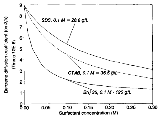
Fig. 2. Decreases of the benzene diffusion coefficient due to its inclusion in micelles of different surfactants.
