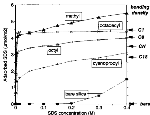
Fig. 3. Amount of adsorbed anionic SDS on 5 different Hypersil silica phases. The arrows on the right point the bonding density of the organic layer. Full characteristics of the phases are listed in Table 3. Data from [25].
